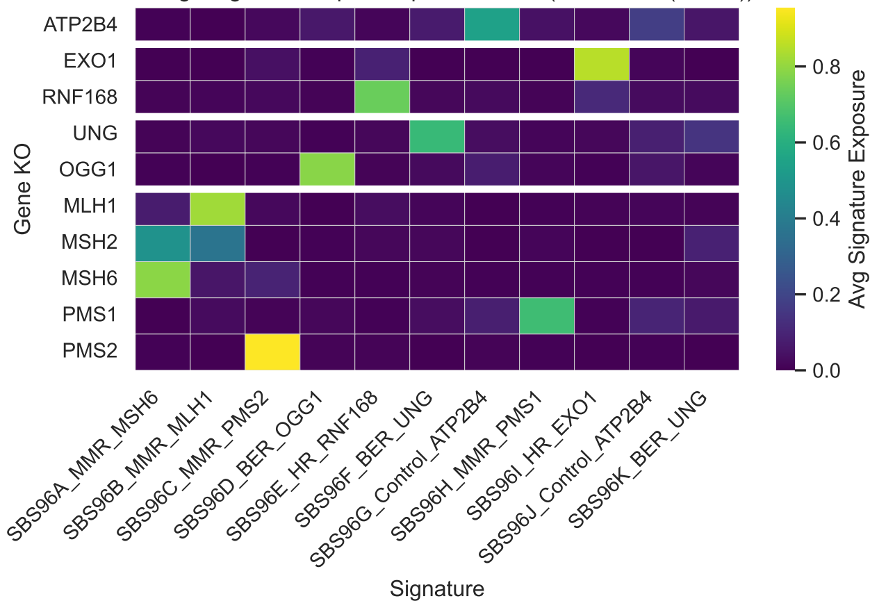
Average Signature Exposure per Gene KO (Gene level (K = 11))
